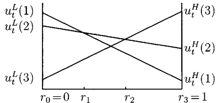
FIGURE 1.—Expected payoff frontier. The diagram depicts the expected payoff of each of three actions as a function of the posterior belief r that the state is H . A rational individual simply chooses the action yielding the highest payoff. Here 2 is an insurance action, and 1 and 3 are extreme actions.
